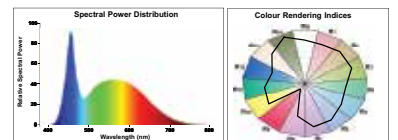
RefLED MR16 V4 865/ 6500K/ Daylight
