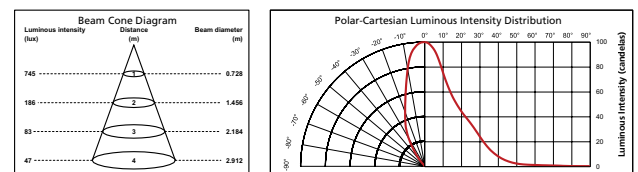
RefLED+ ES50 V2 5W 380lm 40°
