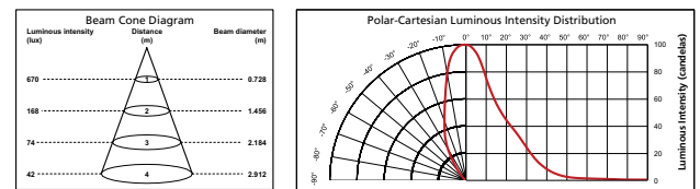
RefLED+ ES50 V2 5W 370lm 40°
