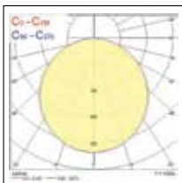
Start Flat Panel LED 600 x 600mm Alto Flusso e Alta Efficienza - 3000K
