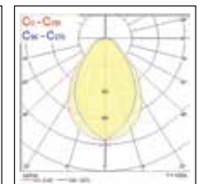
Start Flat Panel LED 1200 x 300mm UGR19 - 4000K
