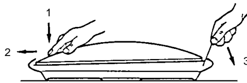
Removing the diffuser. 1. Press down. 2. Push to side. 3. Lever out.
