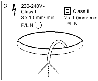
Adjustable Accessory Downlight 2035353 2035354 2035355
