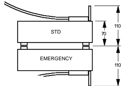
Gear Box - Standard = 180 Dia. x 110 deep Gear Box - Emergency = 180 Dia x 220 deep
