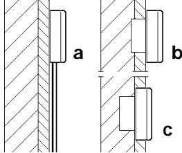
Snap-Fit Wallplate
