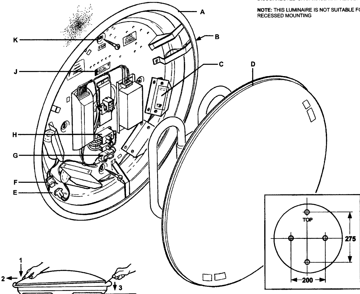
REMOVING DIFFUSER 1. PRESS DOWN 2. PUSH TO SIDE 3. LEVER OUT
