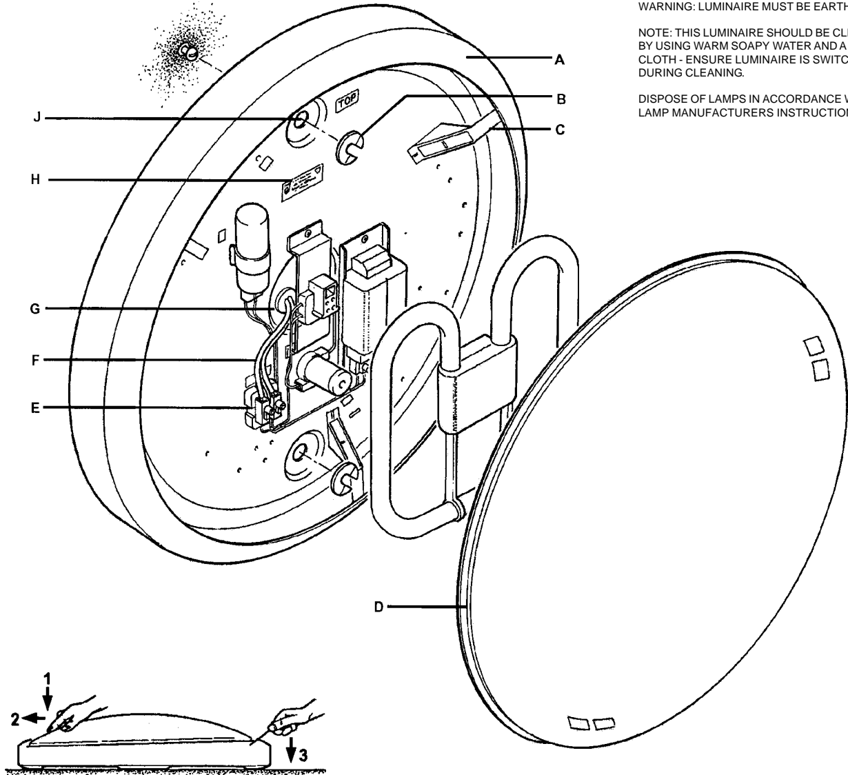
Removing Diffuser 1. Press Down 2. Push to Side 3. Lever Out
