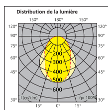
1200 x 300mm - 4,000K
